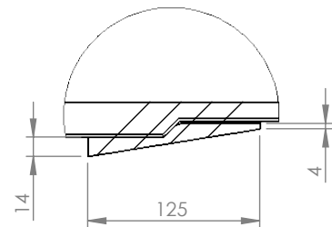
DETAIL D SCALE 1 : 5
